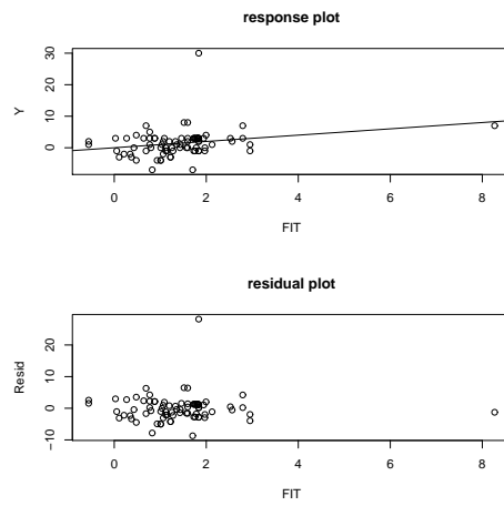
Figure 3. Response and Residual Plots for the AR(2) Model
