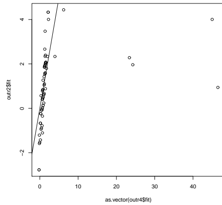
Figure 4. Fitted Values from the Cleaned Data Versus Robust Fitted Values from the Data with 3 Outliers
