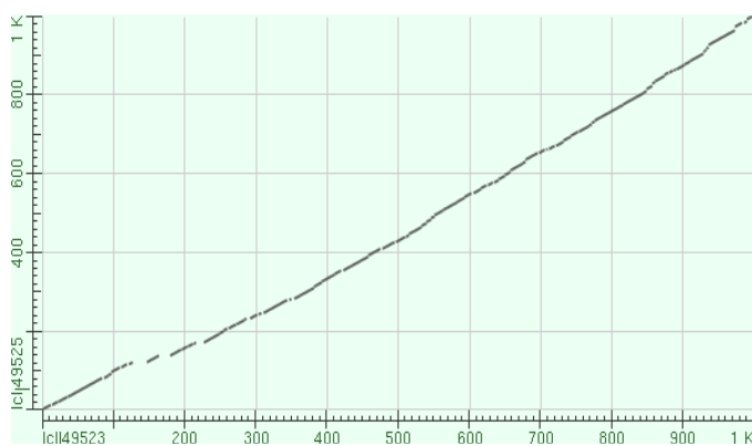
Figure 4. The alignment of the Rhg4 gene between the Forrest B100B10 BAC DNA sequence (x axis) and the Williams 82 56G2 BAC DNA sequence (y axis) from 0 to 1000 bp.
