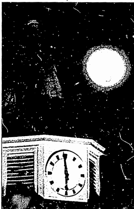
A full moon rises over Pulliam Hall. A few hours later, the moon began moving into the Earth's shadow. The total lunar eclipse lasted until 11:22 p.m. and the full moon was visible again by 12:25 a.m.
