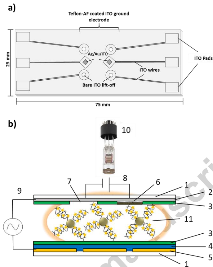
Figure 1. Digital microfluidics and electrochemiluminescence. a) Top-view schematic of device top-plate with four bare circular ITO electrodes (dia. 800 \mu\text{m} ) that serve as ECL working electrodes (WE) and two square Ag/Au/ITO electrodes (560 \mu\text{m} x 560 \mu\text{m} ) that serve as ECL counter/pseudoreference electrodes (CE/RE). The substrate is globally coated with Teflon-AF, with apertures formed above each WE and CE/RE. The ECL electrodes are connected to contact pads through patterned ITO wires, and the remainder of the ITO functions as a ground electrode for DMF operation. b) Cross-section schematic of two-plate digital microfluidic system for ECL detection. (1) Glass substrate (white), (2) Indium tin oxide (ITO) layer (gray), (3) Teflon-AF hydrophobic layer (green), (4) Parylene-C dielectric layer (blue), (5) Chromium array of DMF driving electrodes (yellow), (6) Ag/Au/ITO CE/RE, (7) Bare ITO WE, (8) Working and counter/pseudoreference electrodes connected via a potentiostat, (9) Top-plate DMF ground electrode and bottom-plate DMF driving electrodes connected via an open-source droplet control system, (Fobel et al. 2013) (10) Photomultiplier tube over the top-plate, (11) Droplet containing magnetic beads modified with hybridized DNA oligomers with intercalating labels.
