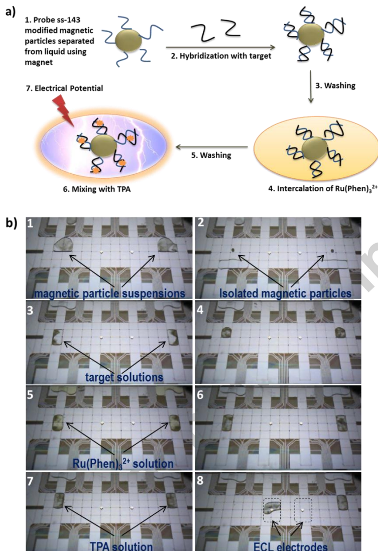
Figure 3. DMF-ECL oligonucleotide hybridization assay. a) Schematic depicting the seven-step DMF protocol developed to detect miRNA-143 by electrochemiluminescence (ECL). b) Frames from the movie depicting the running of two protocols in parallel: (1&2) droplets of ss-143-modified beads are dispensed onto the main platform from reservoir electrodes, followed by magnetic separation of the particles from solution, (3&4) particles are incubated with target sequence droplet followed by wash steps, (5&6) particles are incubated with \text{Ru}(\text{Phen})_3^{2+} solution followed by wash steps, (7) particles are mixed with TPA solution, and (8) finally, one of the two droplets (on the left) is actuated to the ITO WE and Ag/Au/ITO-CE/RE (area inside the dotted rectangle) to measure the ECL. The droplet on the right is queued for a subsequent measurement.
