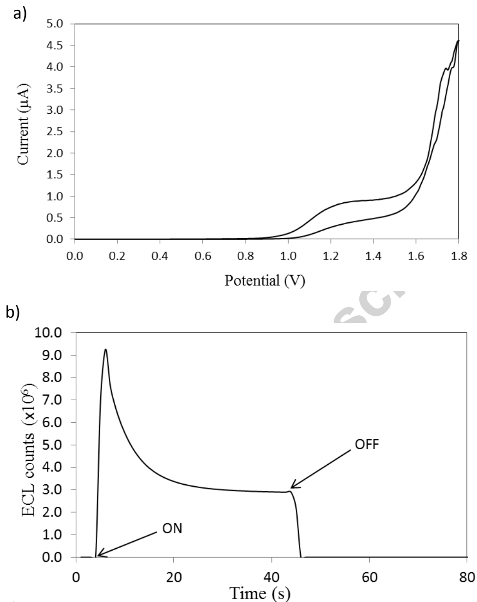
Figure 2. Characterization of DMF-ECL devices. Representative a) cyclic voltammogram (swept from 0 to 1.8 V at 100 mV/s on ITO WE vs Ag/Au/ITO CE/RE) and b) ECL response as a function of time (where “ON” and “OFF” were the times at which 1.5 V as applied and then removed) for a 1:1 mixture of 200 \mu\text{M} [\text{Ru}(\text{Phen})_3]^{2+} and 20 mM TPA in PBS buffer (pH 7.4).
