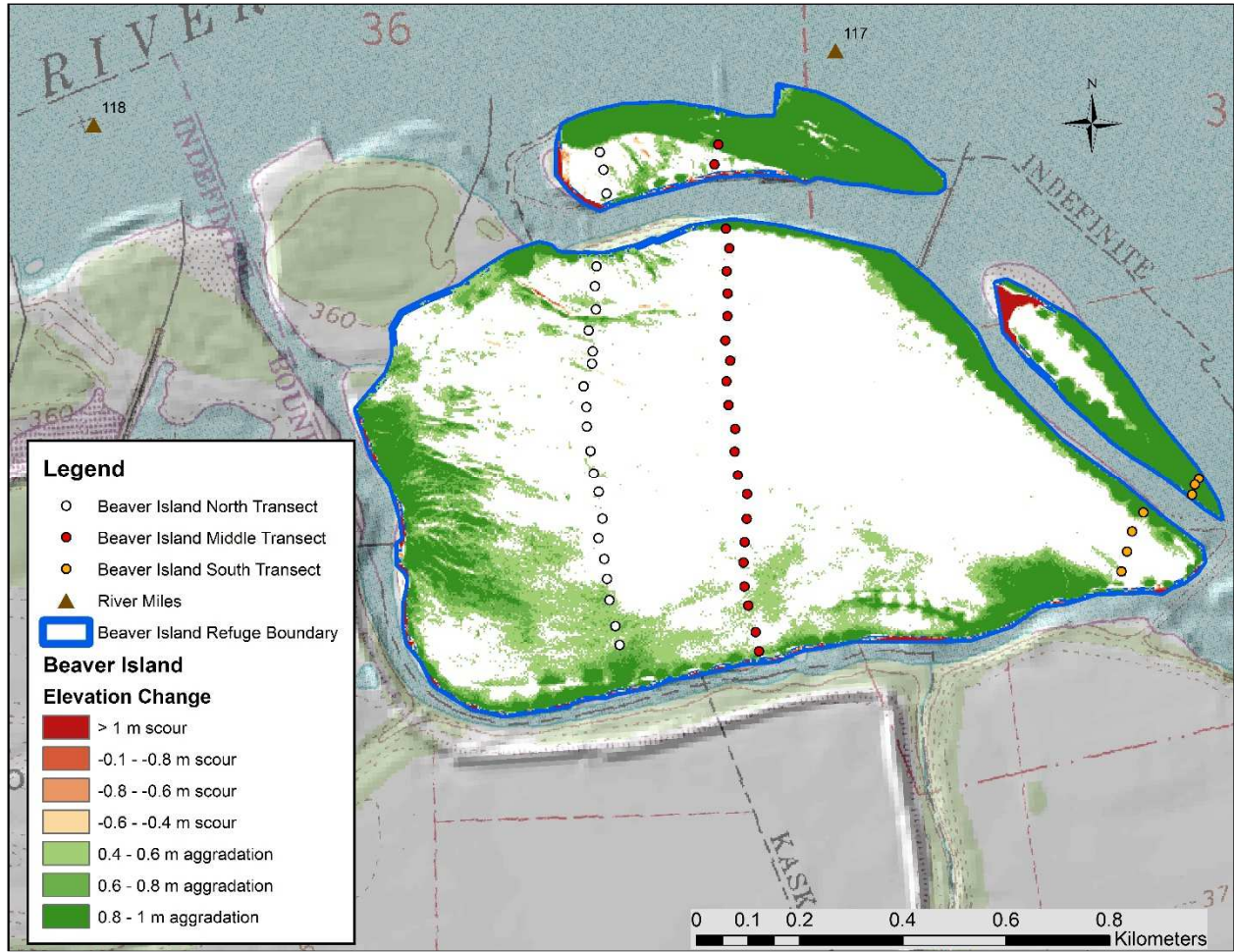
Figure 7: Beaver Island DoD sedimentation depth map with transects and sample locations. Red is erosion/scour, green is aggradation, and white is within the zone of uncertainty in the DoD analysis.
