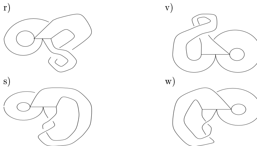
FIGURE 5. Figures (a)-(w) prove Theorem 2
