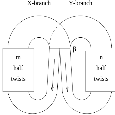
FIGURE 1. Lorenz-like template, L(m, n) , defined
