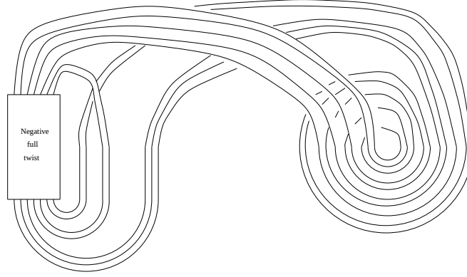
FIGURE 7. Composite knot on L(-2, 0)
