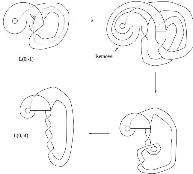
FIGURE 8. L(0, -4) \subset L(0, -1)
