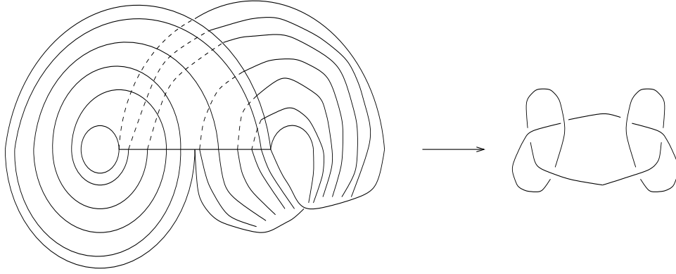
FIGURE 2. A square knot in L(0, -1)
