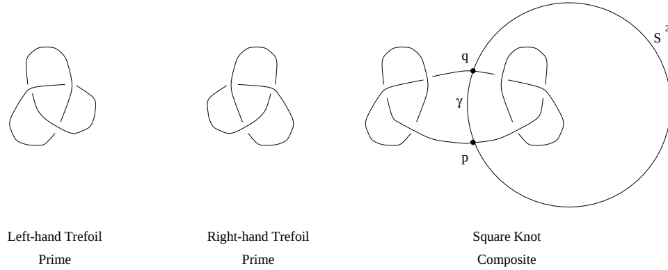
FIGURE 3. A connected sum
