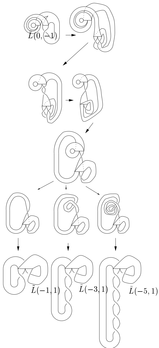
FIGURE 9. Rest of Theorem 3
