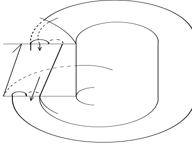
Figure 3.26: The linking number must be at least two.
