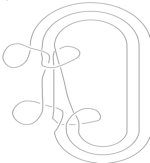
Figure 2.7: c) The Borromean rings.
