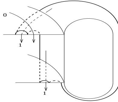
Figure 3.18: Linking number is at least two.
