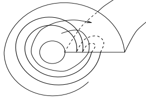
Figure 3.13: Once again we can't guard the U-joints.
