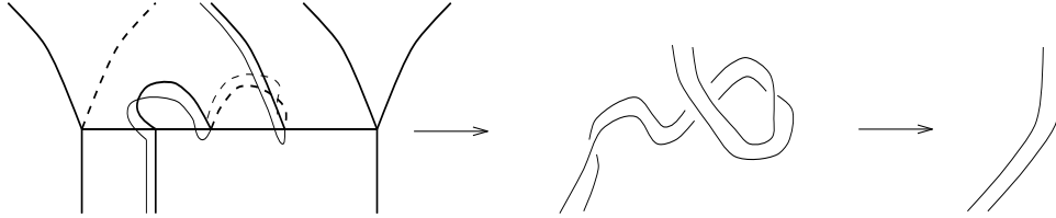
Figure 3.6: U-strings alternate \pm \frac{1}{2} twist at each cusp.
