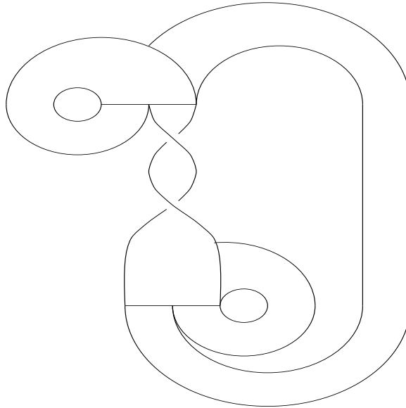
Figure 4.3: \hat{k} on L(0,0)
