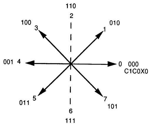
Fig.10 Optimal threshold, C1C0=00.
