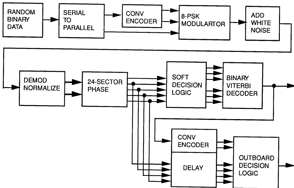
Fig.9 Complete system
