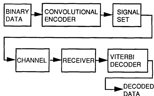
Fig.1 Typical TCM system.
