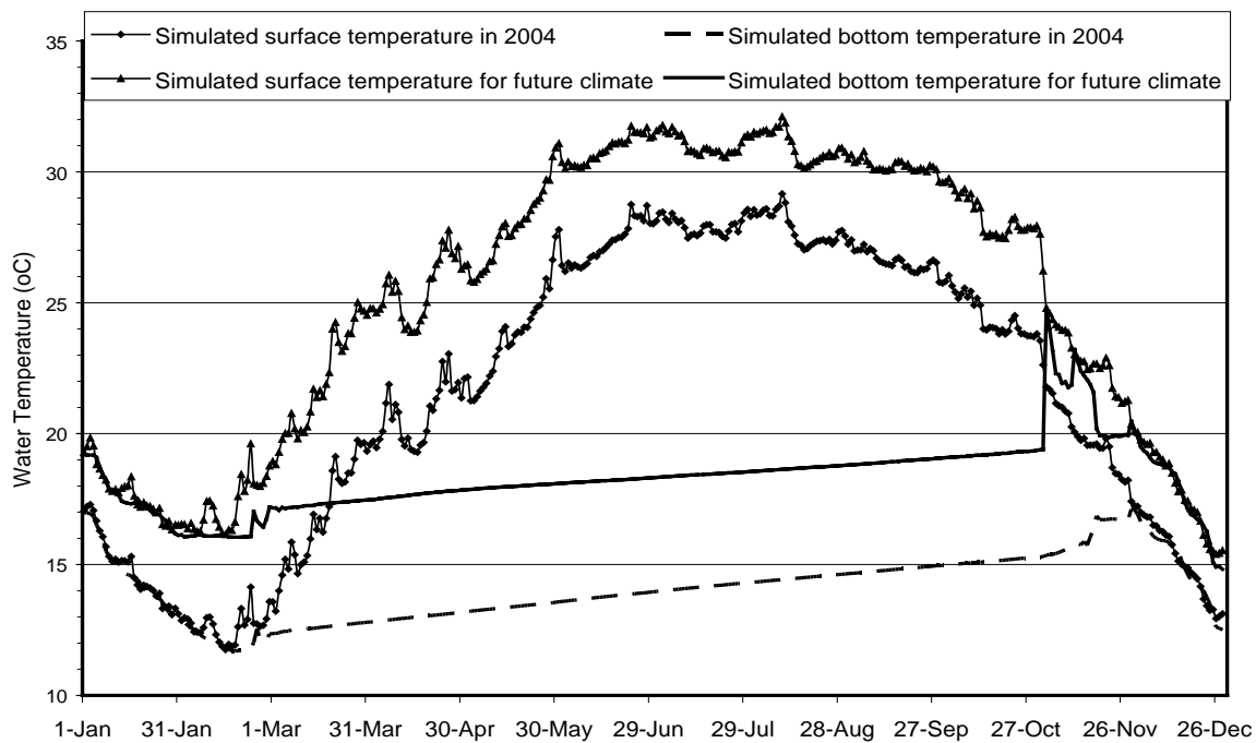
Figure 3. Simulated surface and bottom water temperatures near the dam of Amistad Reservoir under 2004 climate condition and 2\times\text{CO}_2 future climate scenario.
